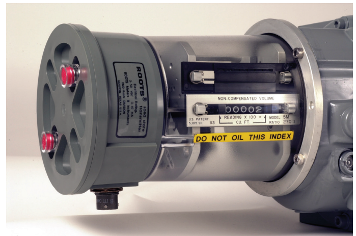
Dresser Series B3-3M175 VRM CEX meter
